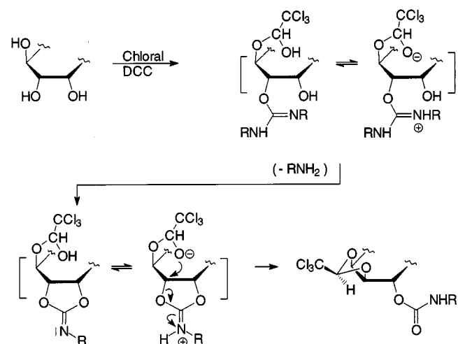
Scheme 1. Mechanism for the epimerisation
