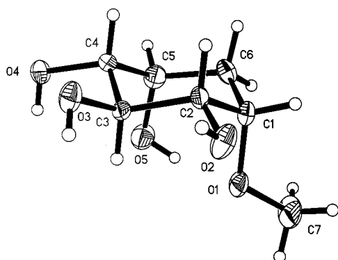
Figure 1. Molecular structure of compound 4 (probability 30%)
