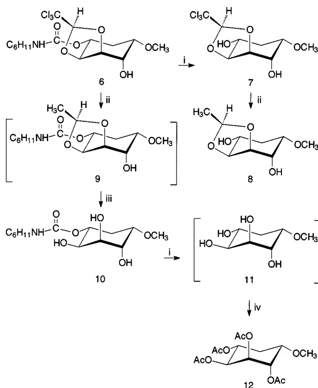
Scheme 3. i: \text{NaOMe}/\text{MeOH} , reflux; ii: \text{Bu}_3\text{SnH}/\text{AIBN} (toluene, argon), reflux; iii: \text{CF}_3\text{COOH} (80%), r.t.; iv: \text{Ac}_2\text{O}/\text{pyridine} , r.t.
