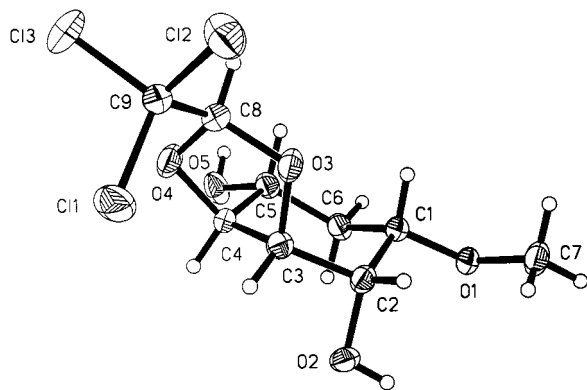
Figure 2. Molecular structure of compound 7 (probability 30%)
